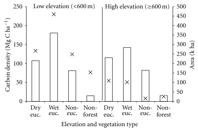
FIGURE 2: Standing-tree C densities and areas by elevation and vegetation type in Tasmanian State forest. Bars denote C density, and crosses denote area.
