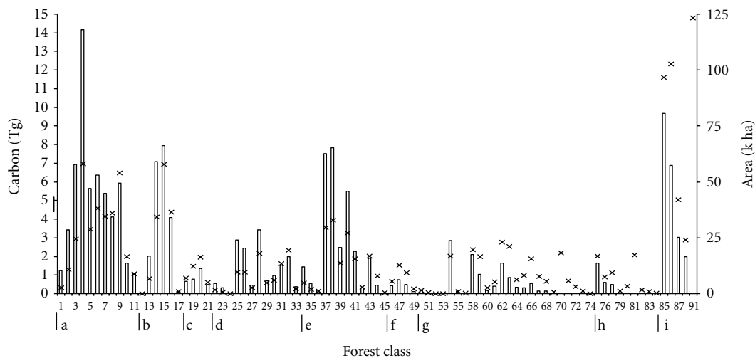
FIGURE 4: Areas and amount of carbon stored in standing trees in Forest Classes in Tasmanian State forest. Forest Classes, 57, 78, 89, and 90 are omitted. For a more complete description of Forest Classes refer to Table 1. Bars denote carbon, crosses denote area. a: mature eucalypt, b: mature eucalypt with unheighted regrowth, c: mature eucalypt with silvicultural regeneration, d: unaged eucalypt regrowth with mature eucalypt, e: pure unaged regrowth eucalypt, f: regrowth eucalypt with silvicultural regeneration, g: even aged eucalypt silvicultural regeneration, h: unstocked, and i: noneucalypt forest.
